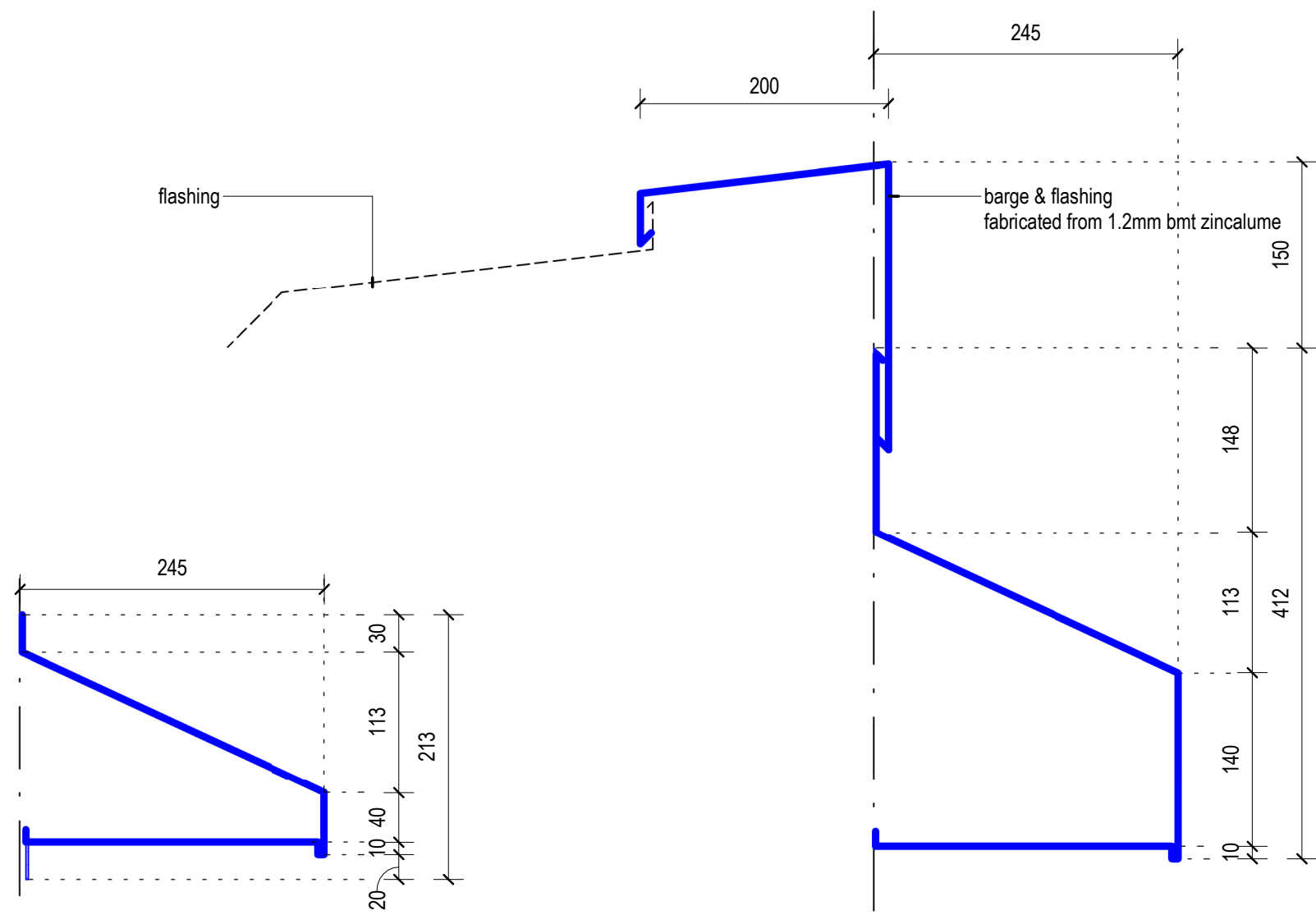
5 Horizontal Flashing - AM-2a & b 1 : 5 Profile
