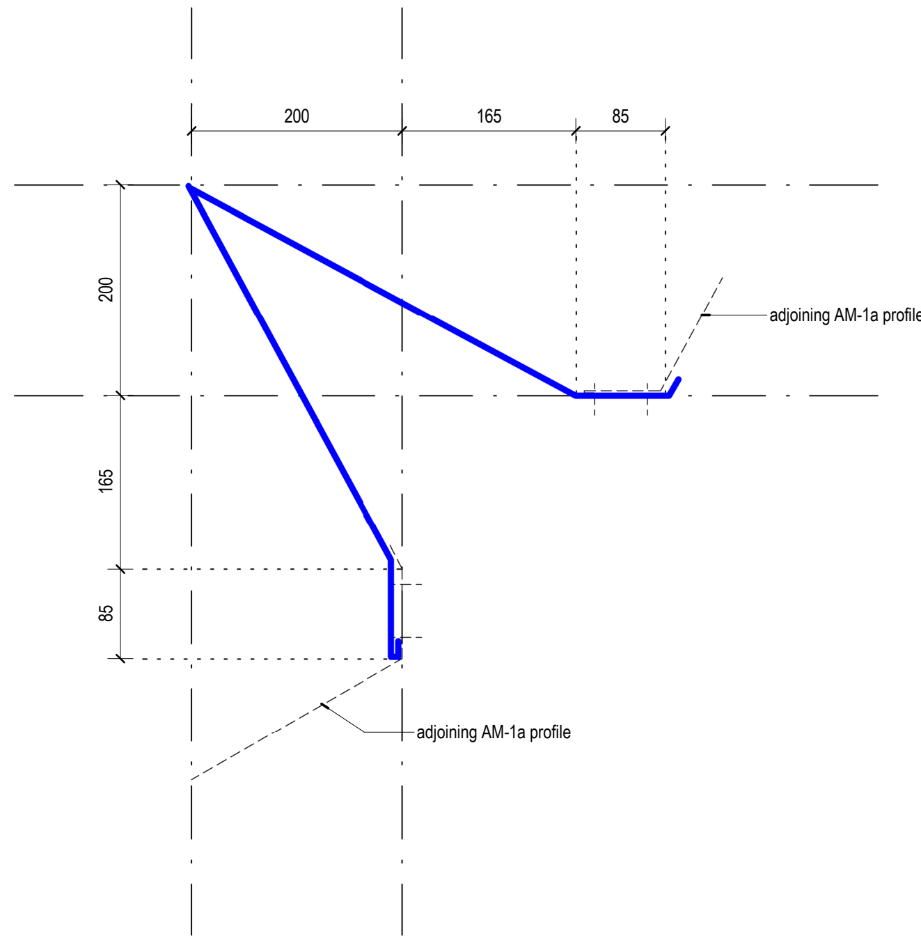
2 Cladding Corner Profile - AM-1d 1 : 5
