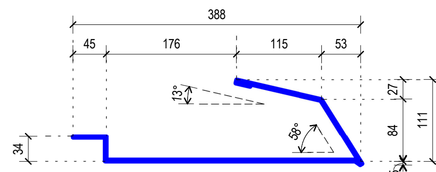
40 AM-4 - Verandah Roof Nosing 1 : 5 Profile
