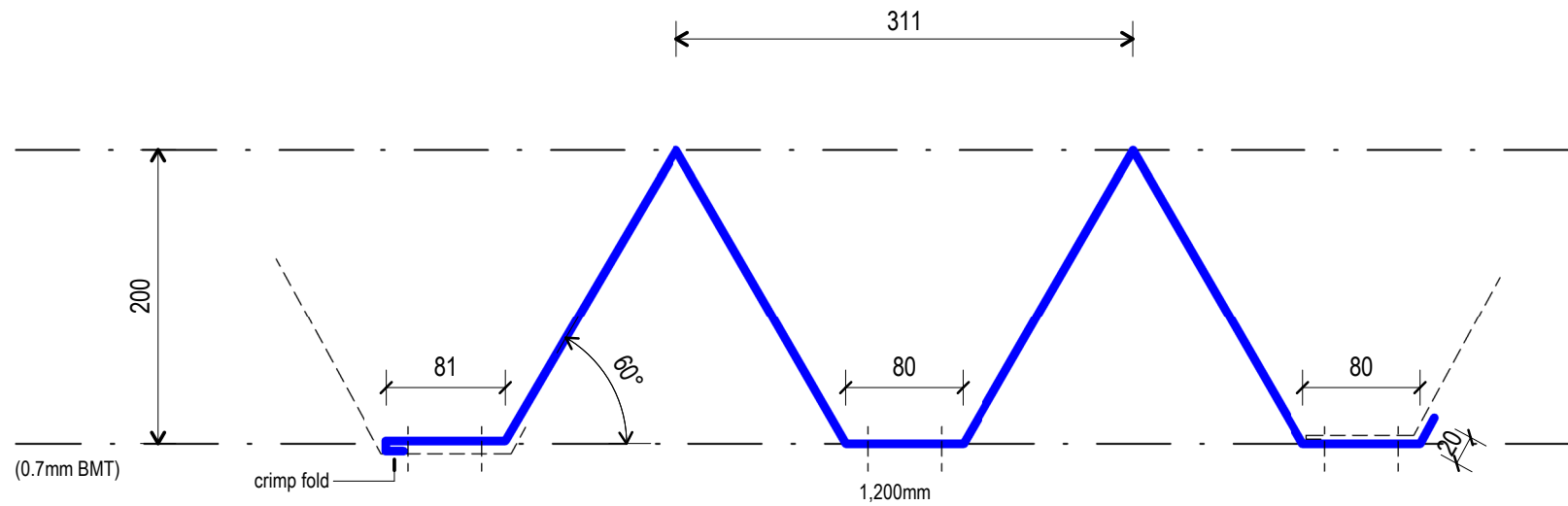
1 Cladding Profile - AM-1a 1 : 5
