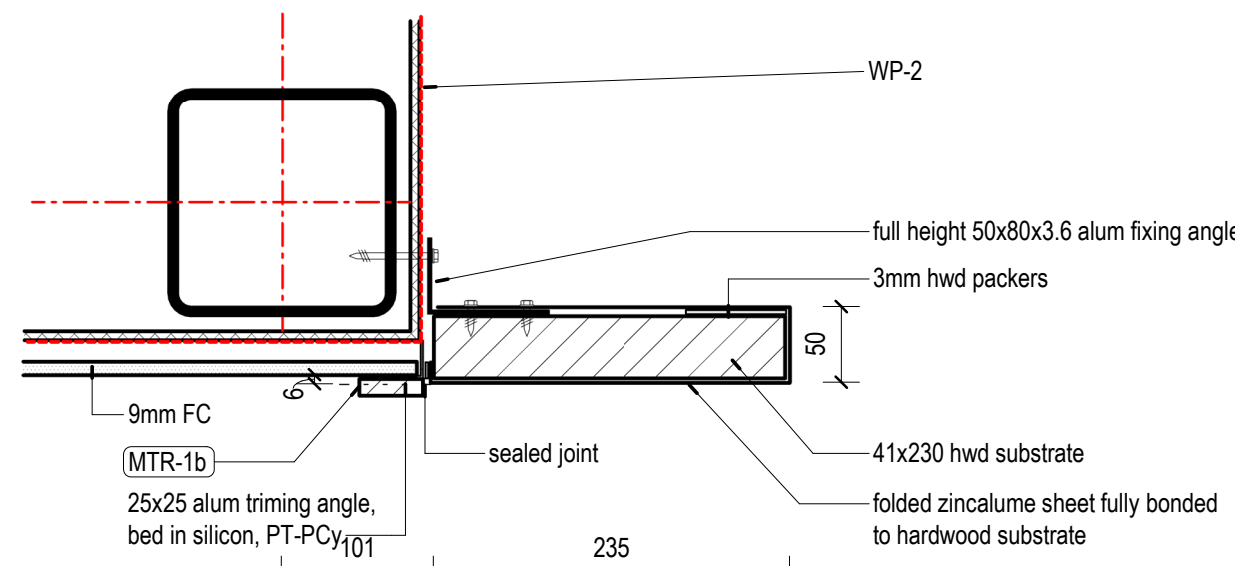
7 Vertical Flashing - AM-3 1 : 5 Profile
