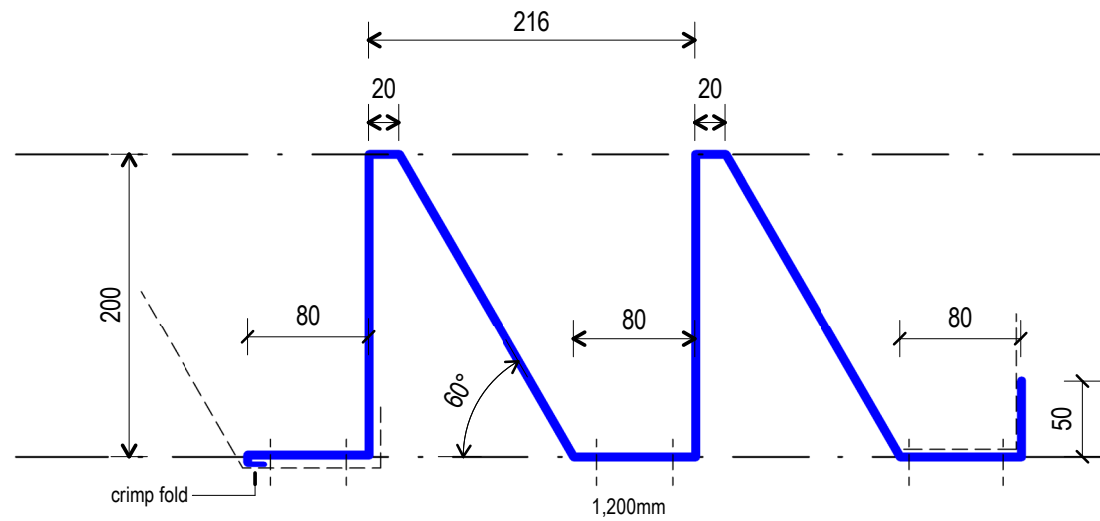
3 Cladding Profile - AM-1b 1 : 5 AM-1c mirror reverse
