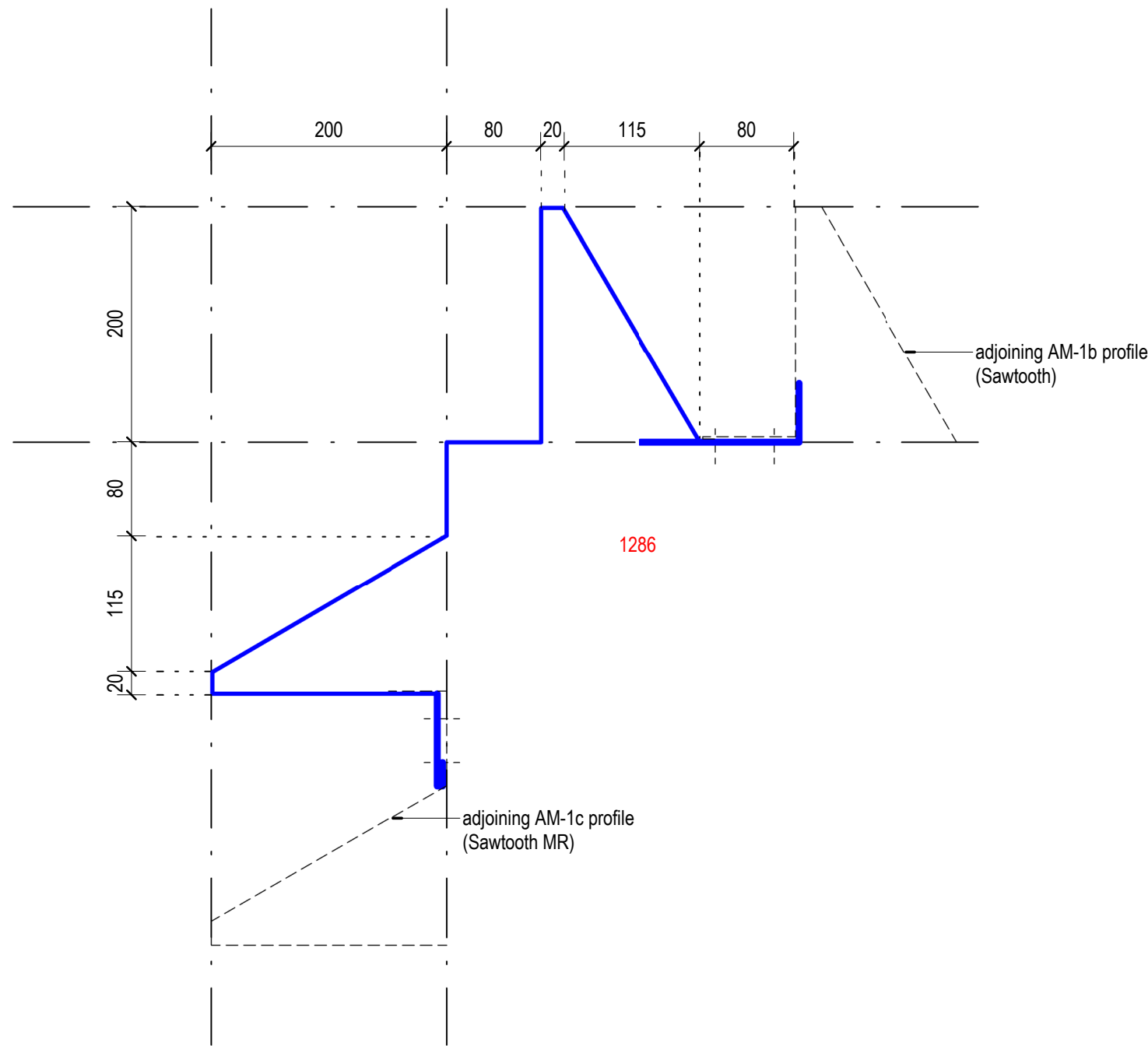
4 Cladding Corner Profile - AM-1e 1 : 5 AM-1f mirror reverse
